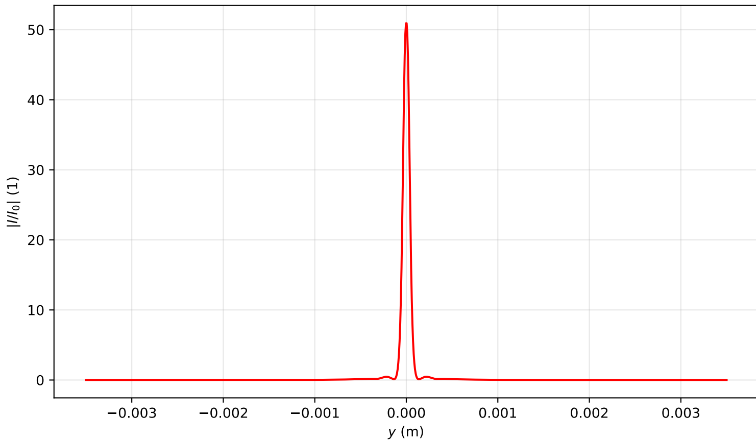
Intensity profile I(x=0, y, z=1.194)/I_0 , P_{in}=2.0P_{cr} , artificial time
